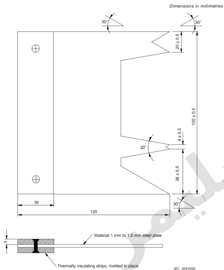
Figure 3 – Flame height gauge
