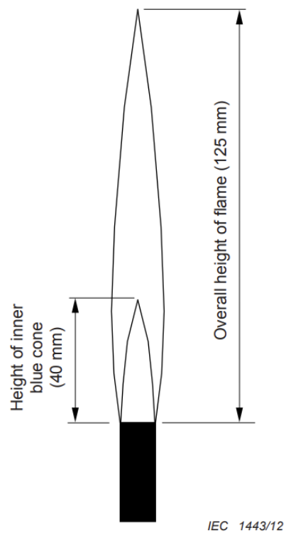
Figure 1 – Flame dimensions
