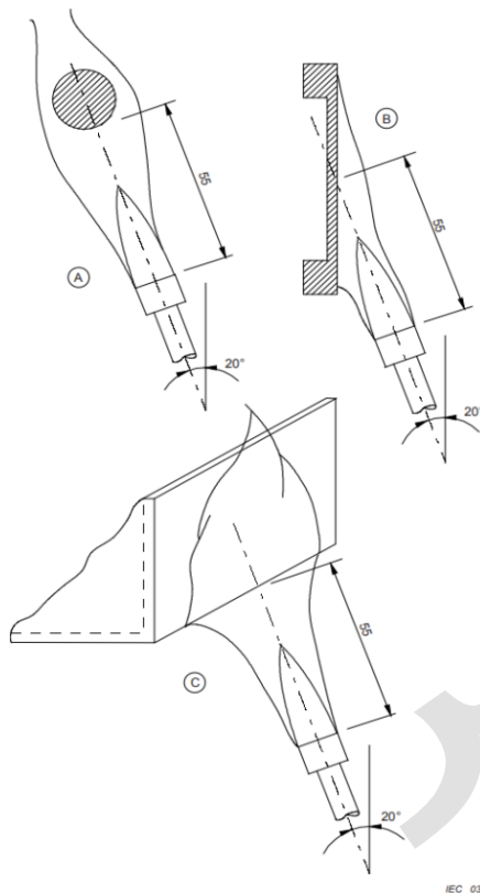
Figure D.1 – Examples of test arrangements
