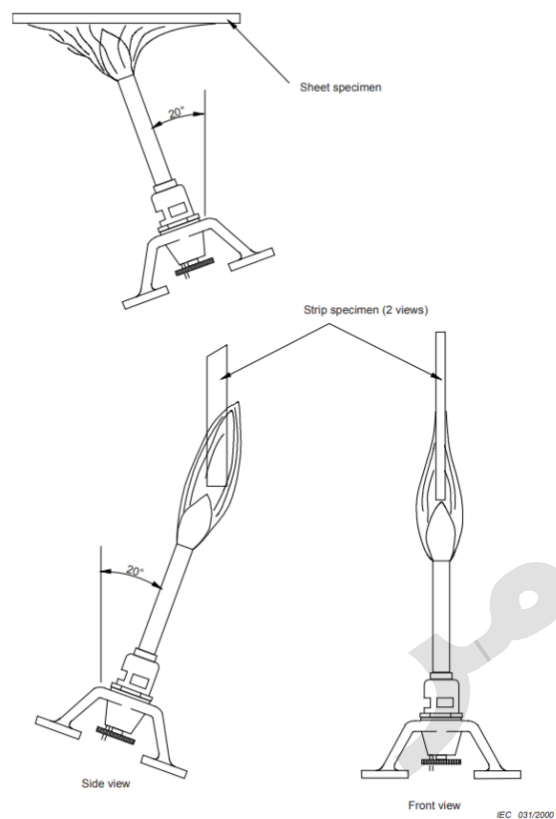
Figure E.1 – Examples of test arrangements
