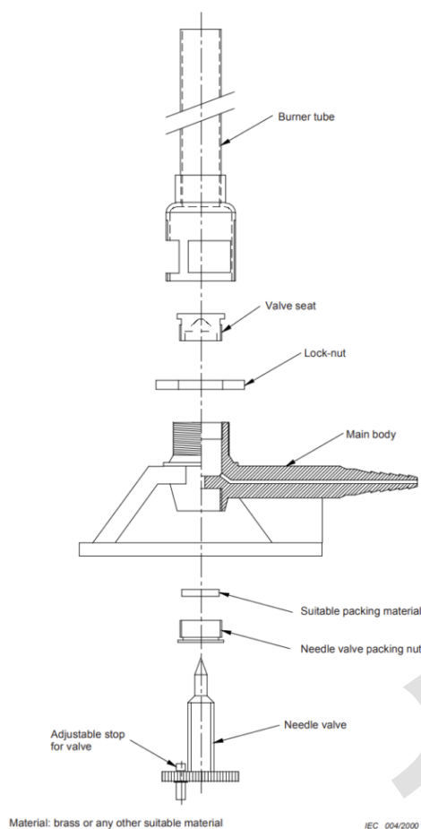
Figure A.1 – General assembly and details
